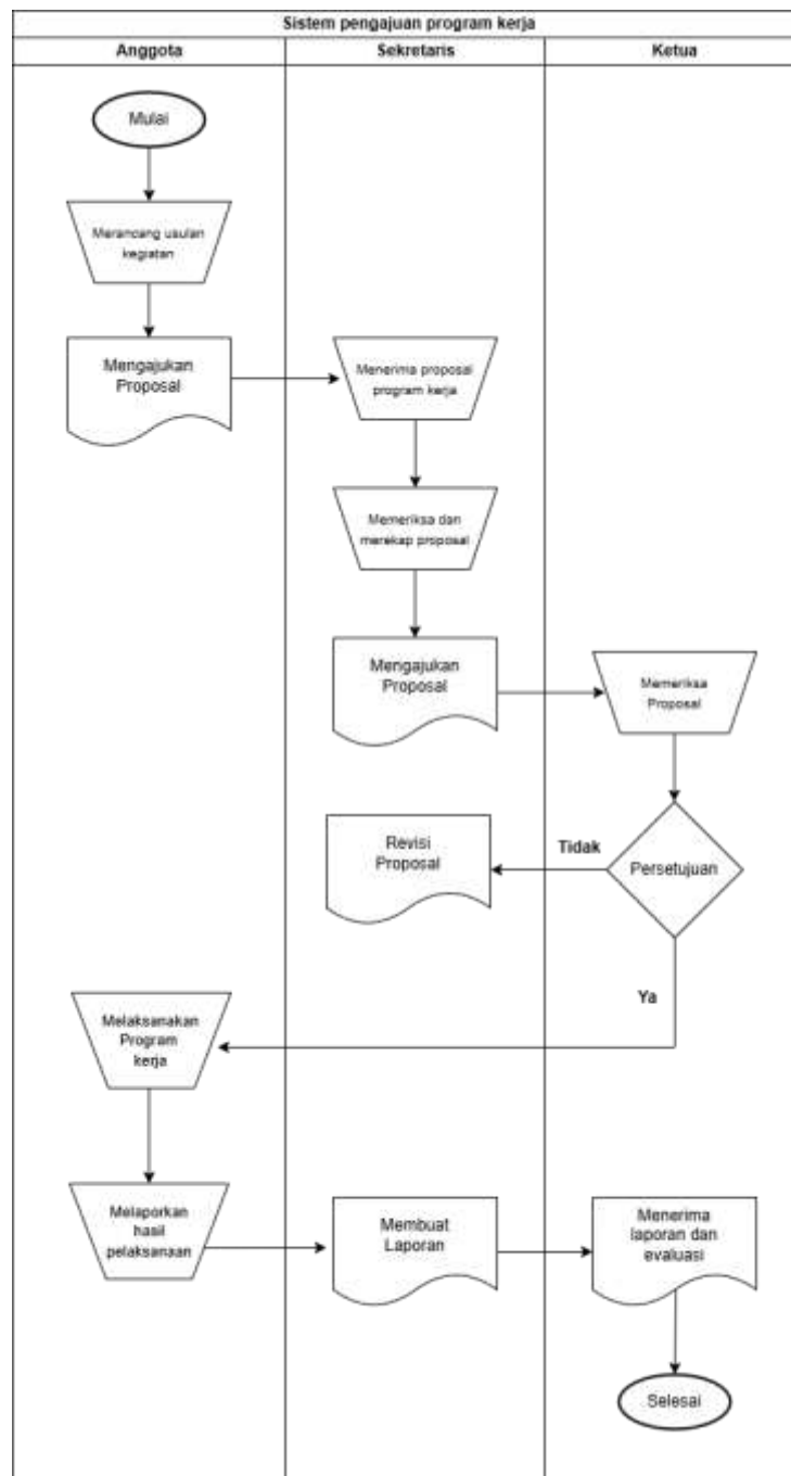
Gambar 4.1 Flowmap Sistem pengajuan program kerja
