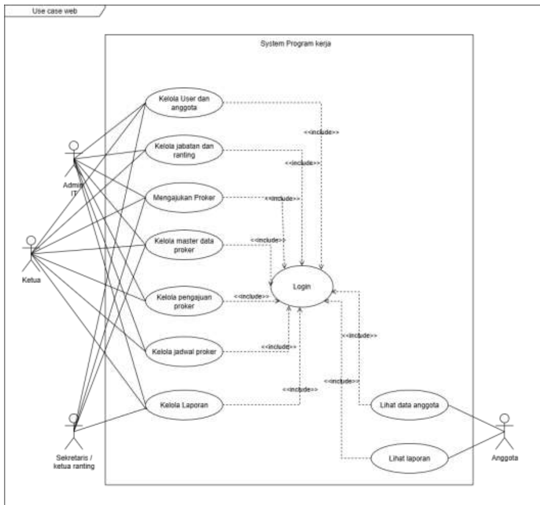
Gambar 4.2 Usecase Diagram
